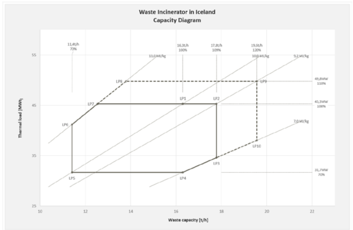
Figure 9. Capacity diagram for a single line plant with a capacity of 16.3 t/h. Nominal Calorific Value = 10 MJ/kg.
