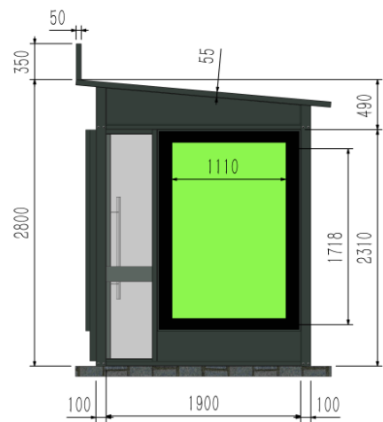
right view
